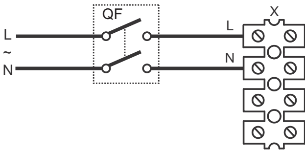
Wiring diagram 16
