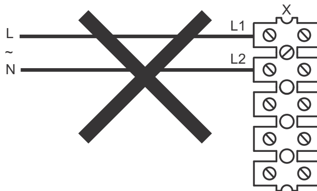
Wiring diagram 4
