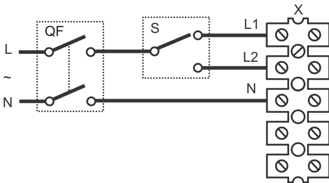
Wiring diagram 3
