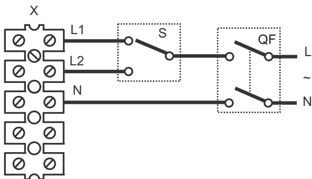
Wiring diagram 7
